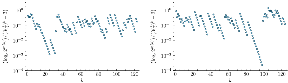
Fig. 3. Length of the ternary representation of 2^{\rho_\chi} (being approximately \rho_\chi \log_3 2 ) as a fraction of the expected number of rolls of three-sided die required to generate an uninterrupted sequence of k non- \chi digits (that average roll count being 3(\frac{3}{2})^k - 3 ).
