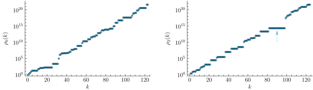
Fig. 2. Plots of \rho_0 (resp., \rho_2 ), defined as the smallest integer n such that the digit 0 (resp., 2) occurs nowhere in the last k ternary digits of 2^n . The arrow points to the instance where \rho_2(k) = 201015414581294 for all 82 \leq k \leq 98 .
